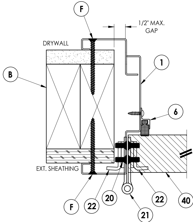
1 HORIZONTAL CROSS SECTION 3 Wood Stud Installation
