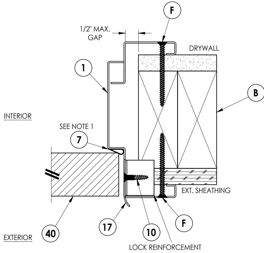
2 HORIZONTAL CROSS SECTION 3 Wood Stud Installation
